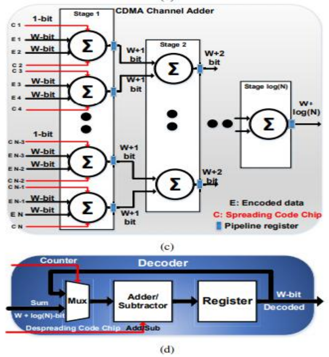
Figure 2. (c) ACDMA channel adder, (d) ACDMA decoder
