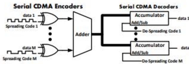
Figure 1. Conventional CDMA crossbar .
