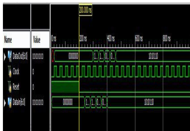
Fig 6. Decoder output
