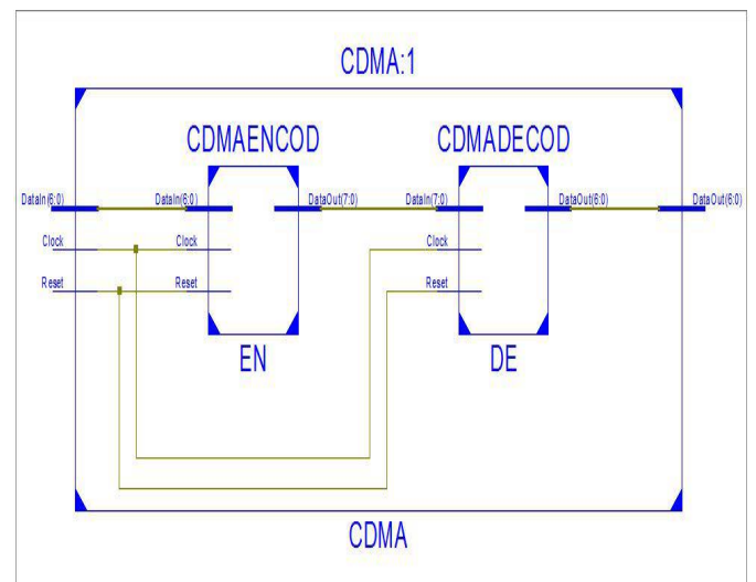
Fig 4. RTL Schematic
