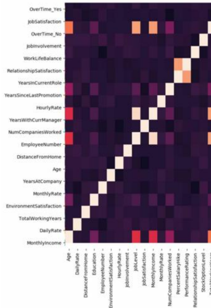
Figure 1. Correlation between various features
