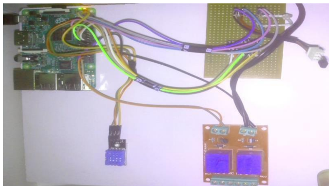
Figure 7: WSN node.
