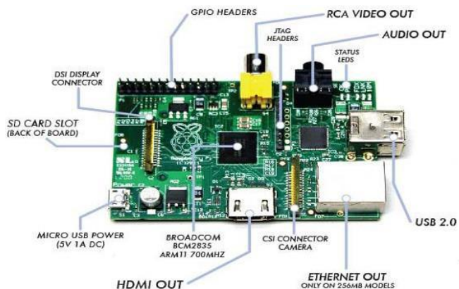
Figure 5: Raspberry Pi.
