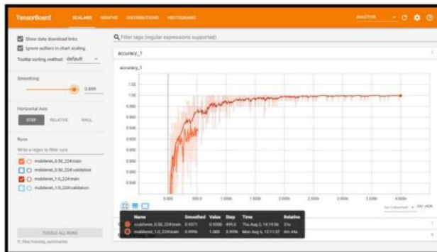
Fig. 11. Graph of 0.50 vs 1.00 MobileNet
