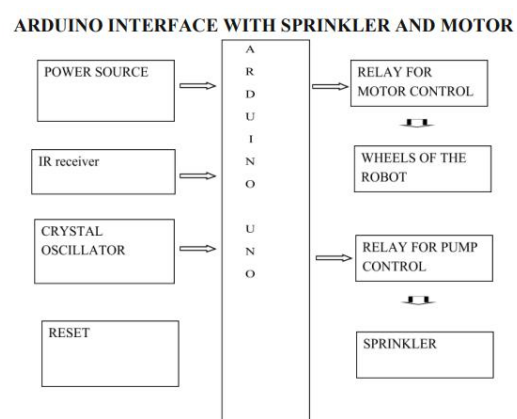
Figure.5.1. Arduino Interface with Sprinkler and Motor
