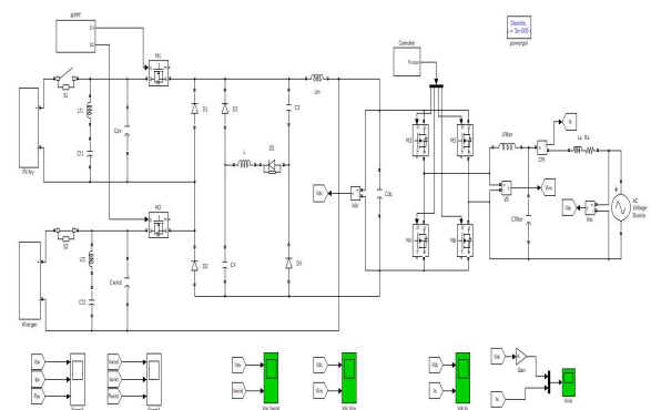
Fig.4.3. Wind power applied.
