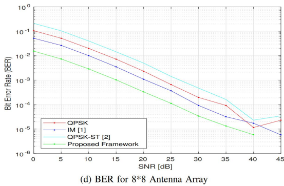
Fig. 2: BER Analysis Results
