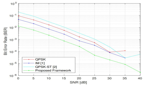
(a) BER for 2*2 Antenna Array
