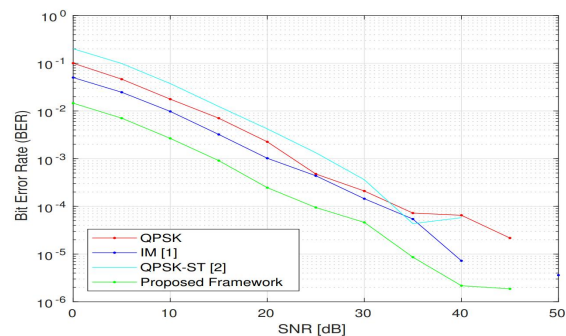
(b) BER for 4*4 Antenna Array
