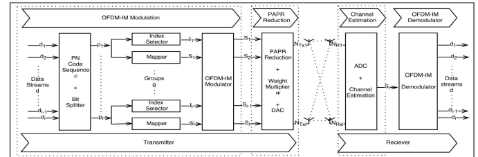
Fig. 1: Proposed End-to-End Framework
