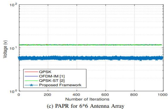
(c) PAPR for 6*6 Antenna Array
