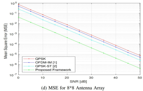
Fig. 3: MSE Analysis Results
