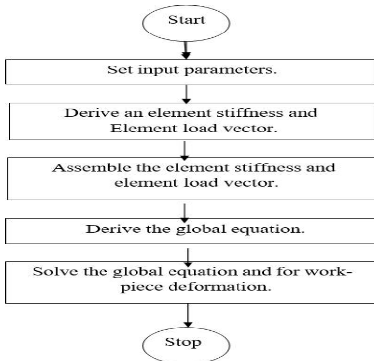
Figure4Flowchartofstaticanalysis
