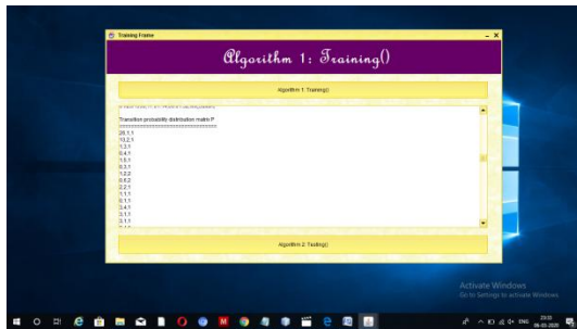
Transition probability distribution matrix p
