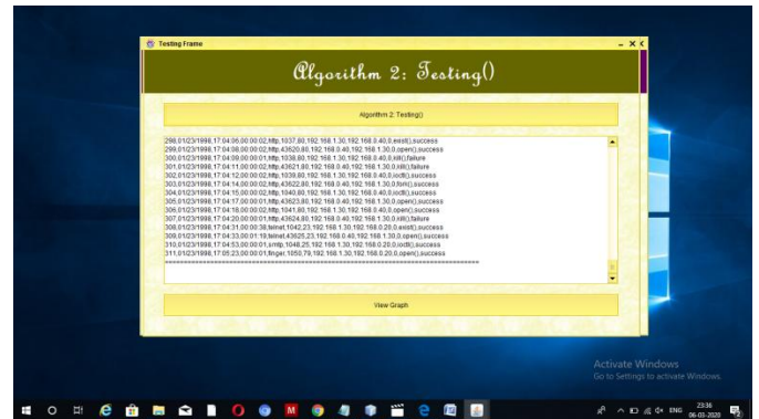
Testing Algorithm
